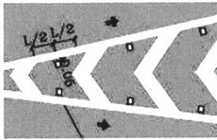
Tacha branca monodirecional
